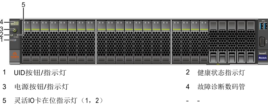
图 2-8 8x2.5 SAS/SATA+12x2.5 NVMe 硬盘配置前面板指示灯和按钮
